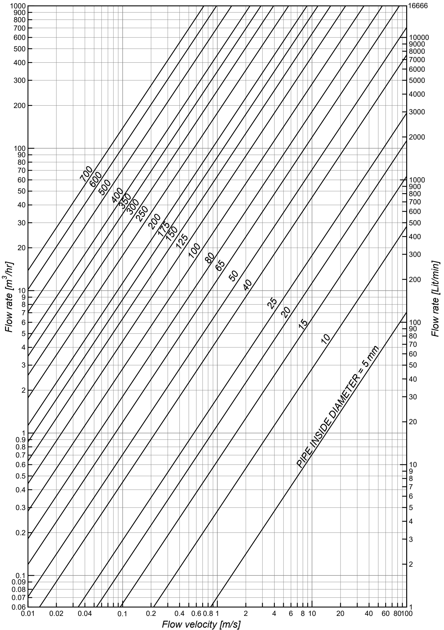
Figure.1 The relation between flow velocity and flow rate at each pipe size
