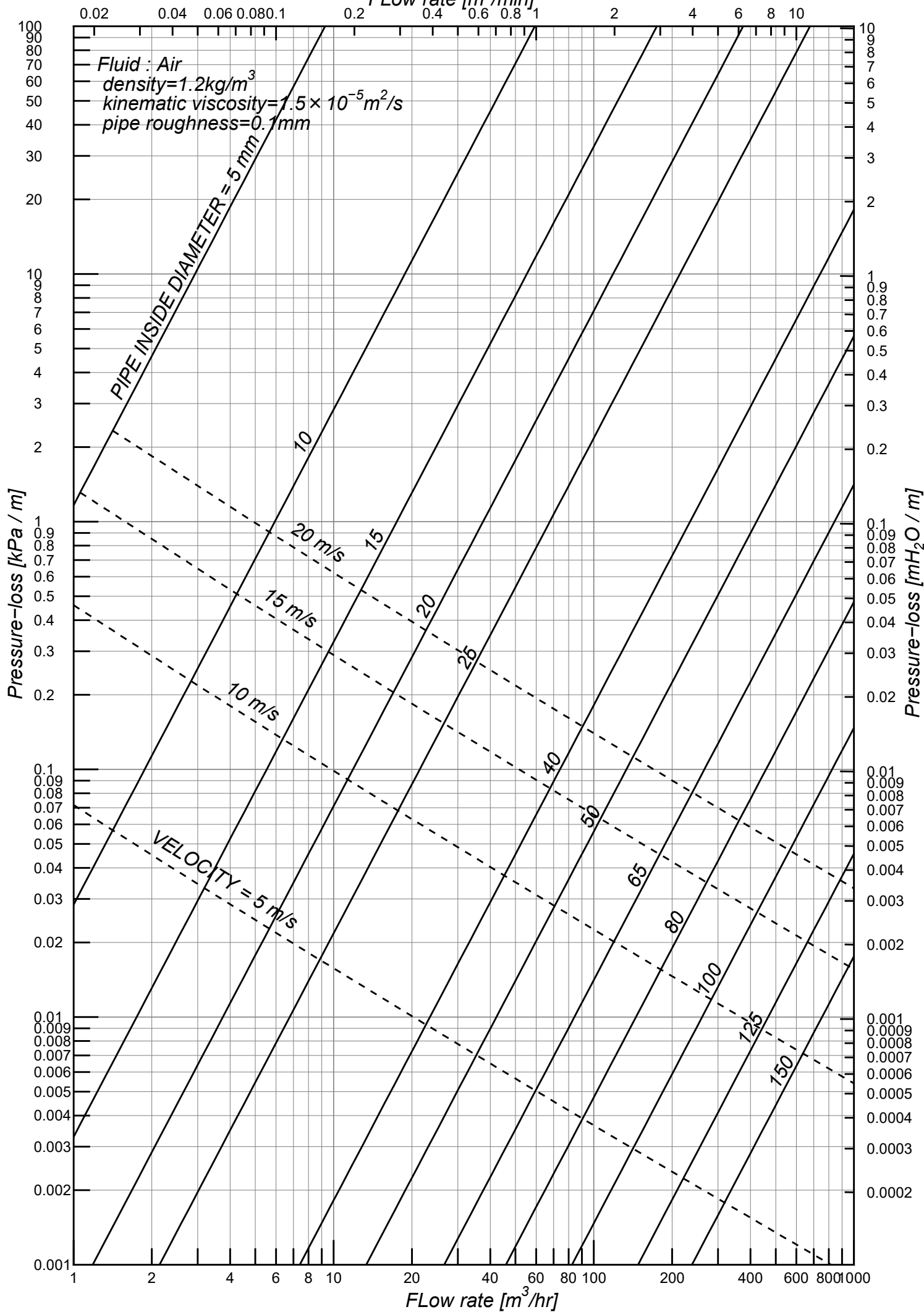
Figure.2 The relation between Pressure-loss and Flow-rate at each pipe size written by Ellery Q
