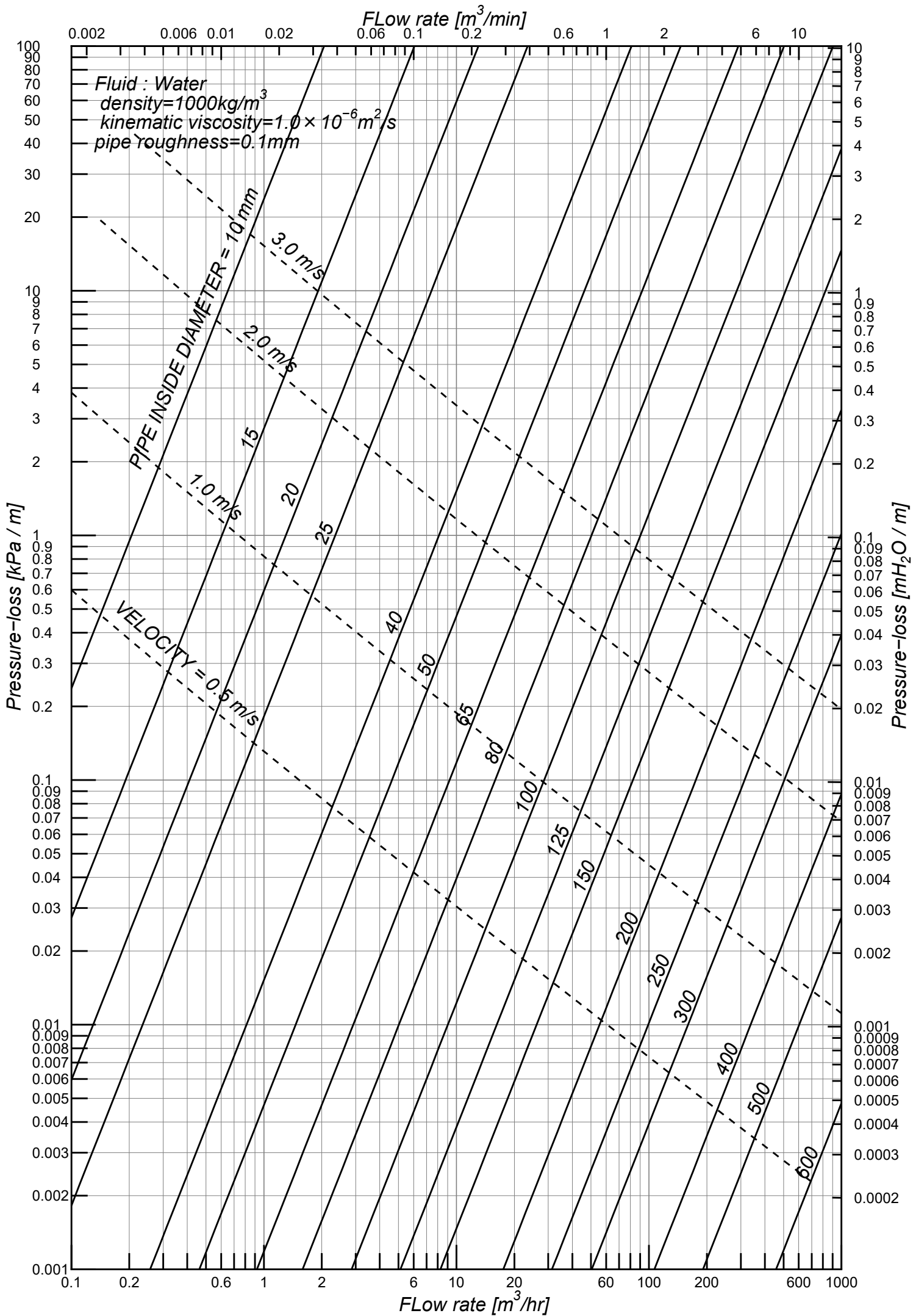
Figure.3 The relation between Pressure-loss and Flow-rate at each pipe size
